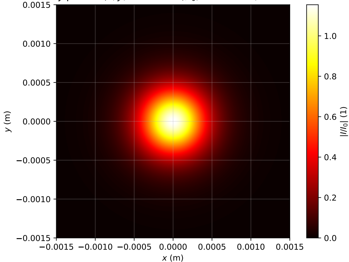
Intensity profile I(x, y, z = 1.751m)/I_0 , P_{in}=0.7P_{cr} , artificial time
